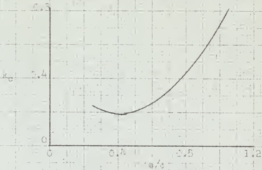
FIG. 12 -- EFFECT OF GAP/CHORD RATIO ON RESISTANCE COEFFICIENT.
